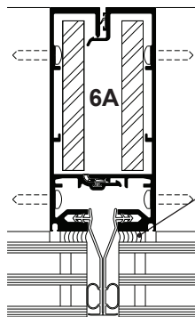
OPTIONAL STEEL REINFORCING AS REQUIRED
