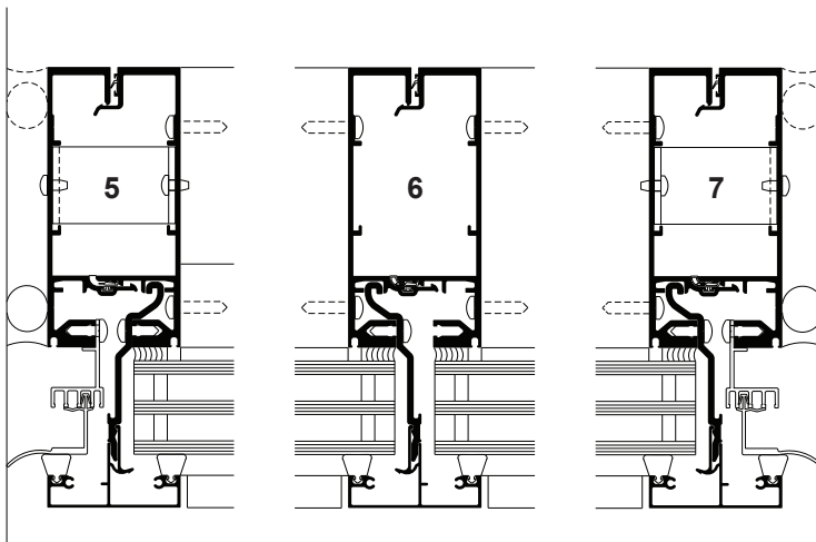
TYPICAL ELEVATION (CAPTURED SYSTEM)
